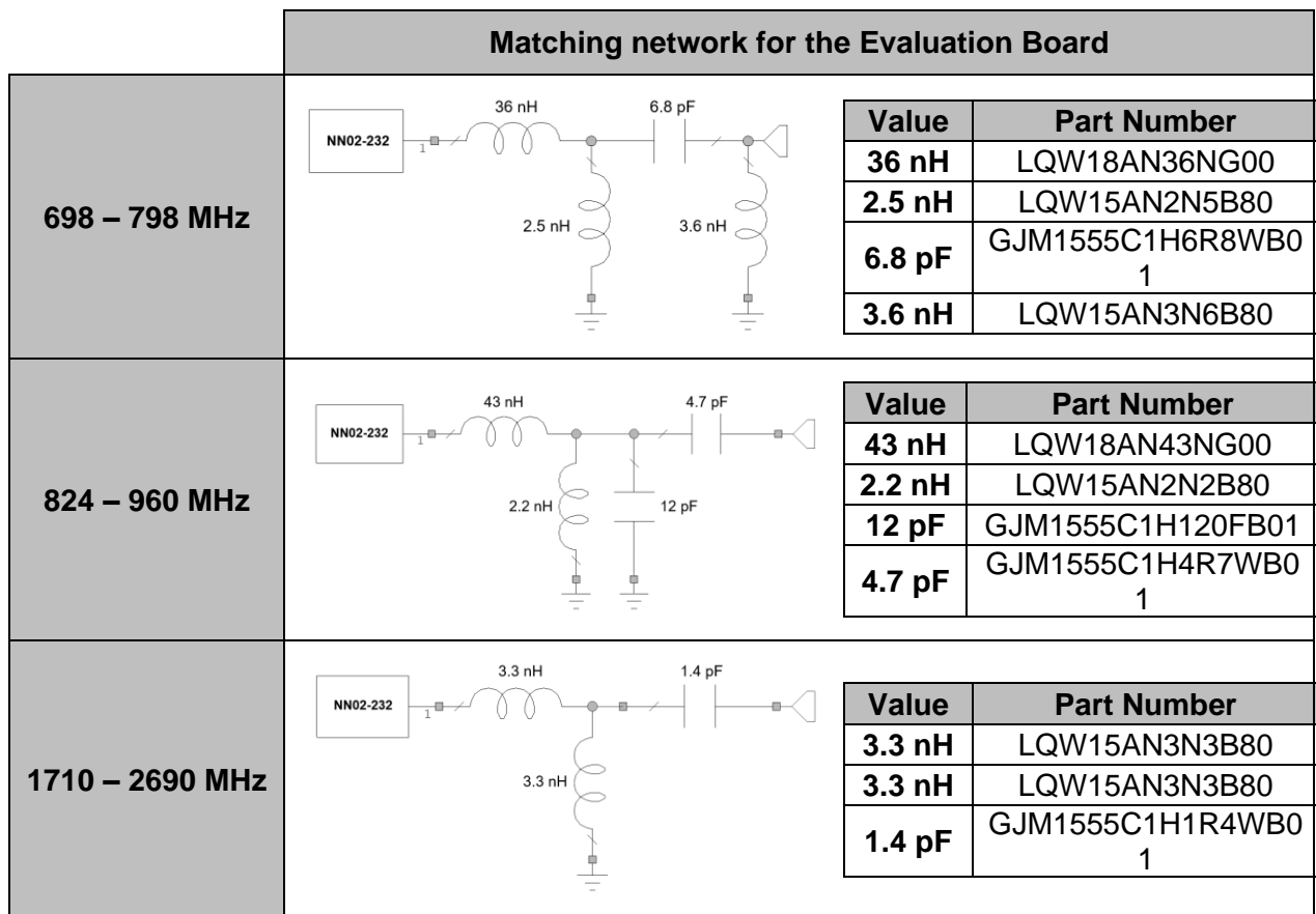
Figure 2 – Matching networks implemented in the Evaluation Board 3 ports (Figure 1).
