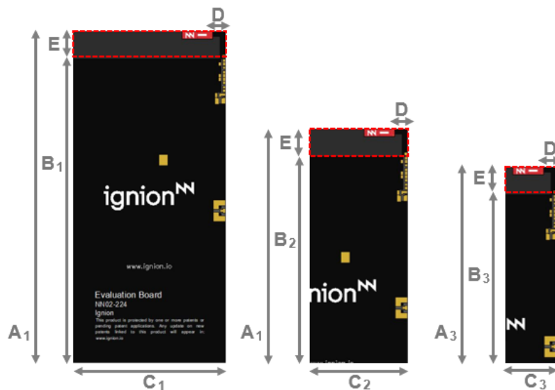
Figure 1 – Evaluation Board with different size dimensions providing operation from 863 MHz to 928 MHz and from 2400 MHz to 2500 MHz.
