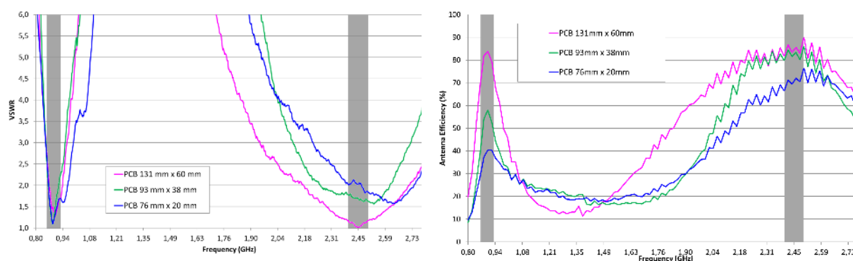
Figure 2 – VSWR and Total Efficiency for the 863 – 928 MHz and 2400 – 2500MHz from the evaluation board (Figure 1).
